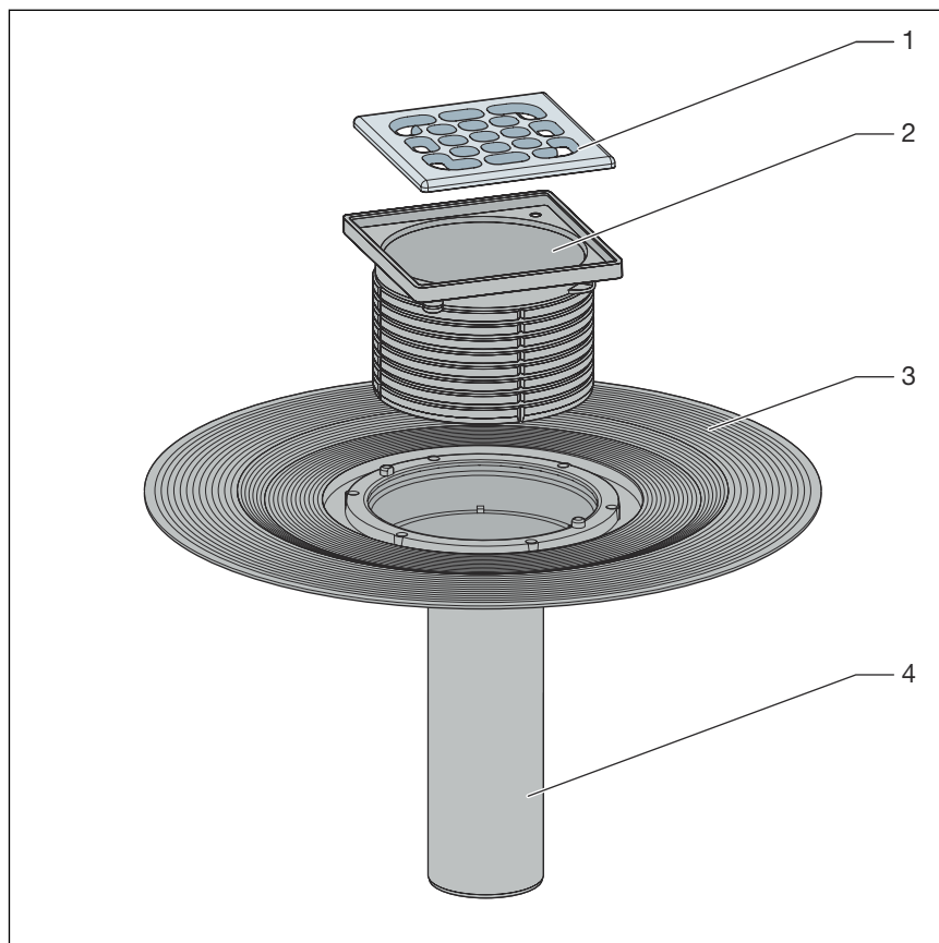
Fig. 1: Components balcony / terrace drain model 4944.2
